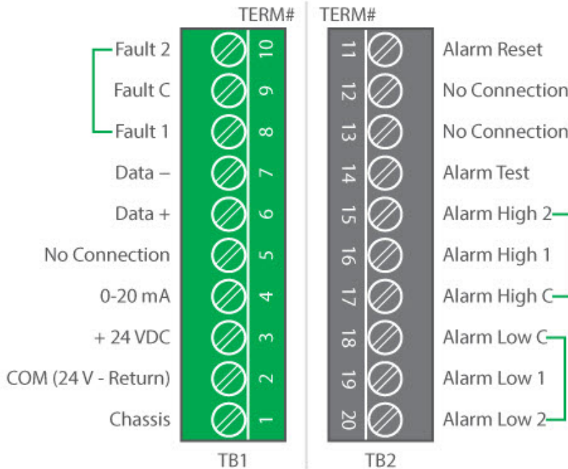
Figure 17 Field Terminations
