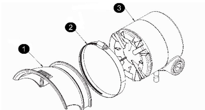
Figure 20 Exploded View
